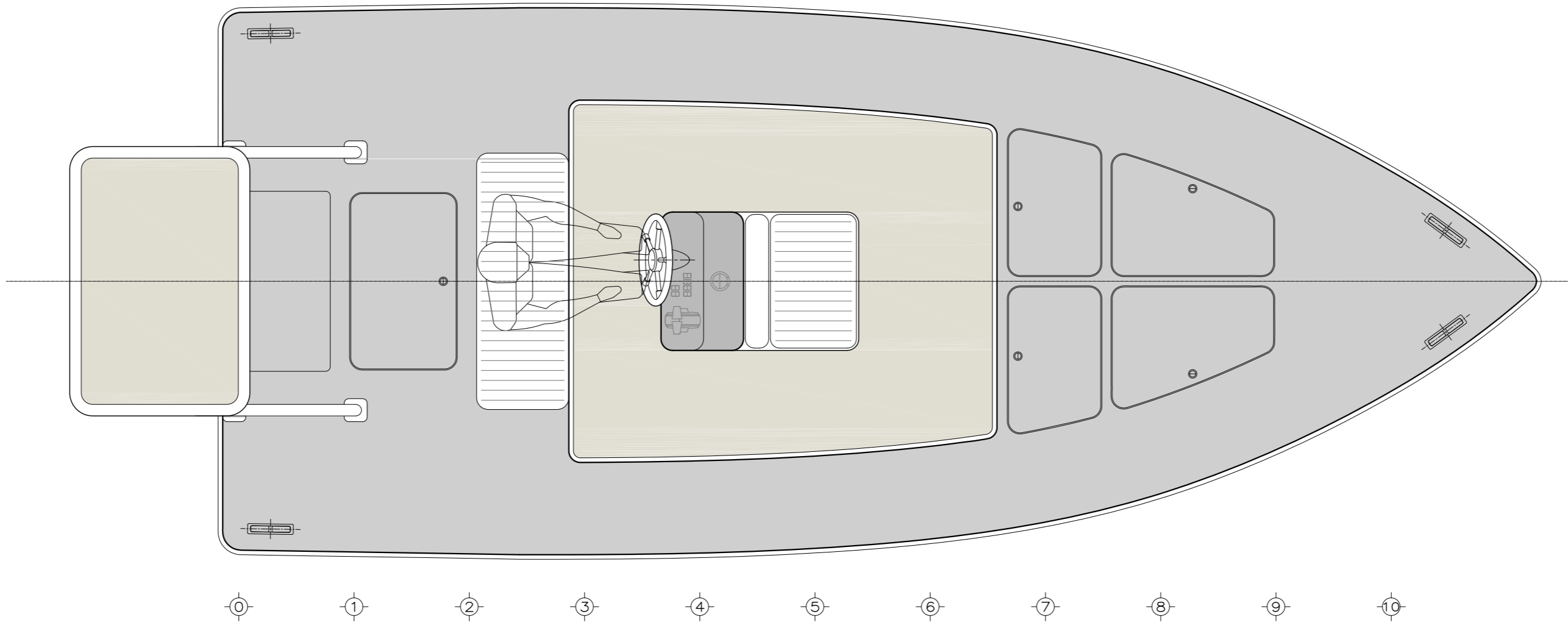
TOP VIEW SCALE 1:20
